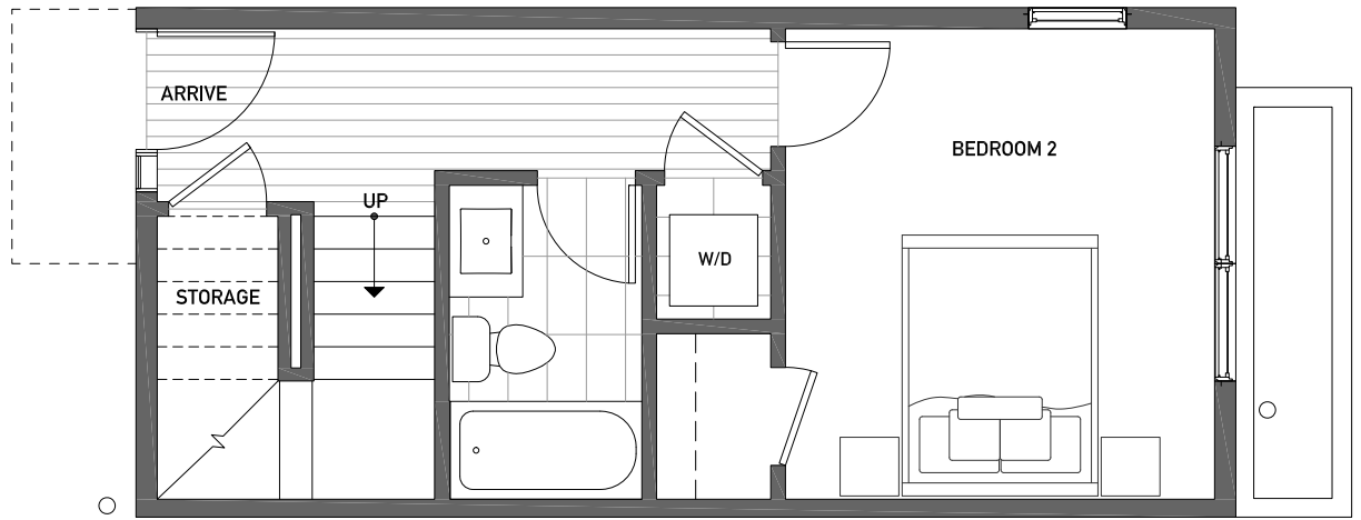
FIRST FLOOR
