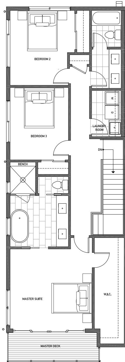
THIRD FLOOR
