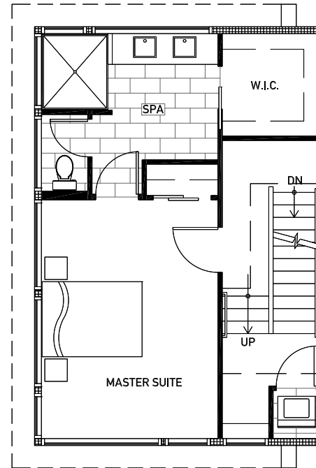
Floor Three
