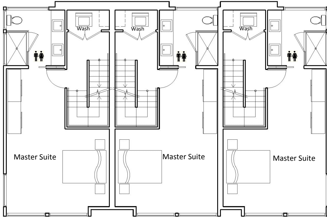
THIRD FLOOR
