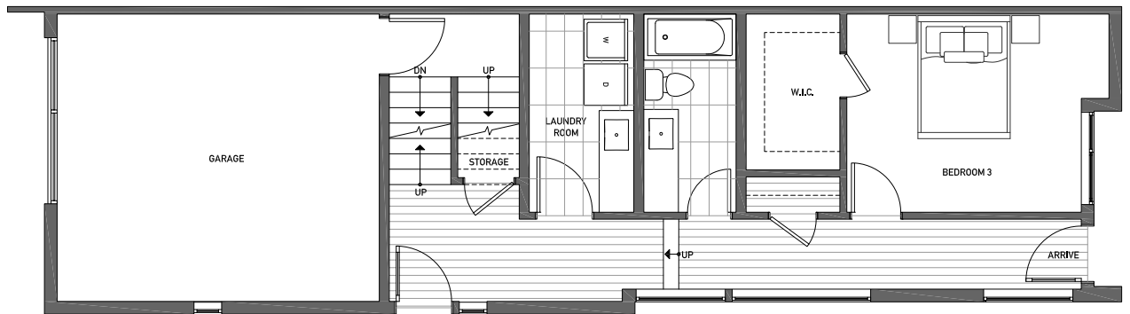
FIRST FLOOR
