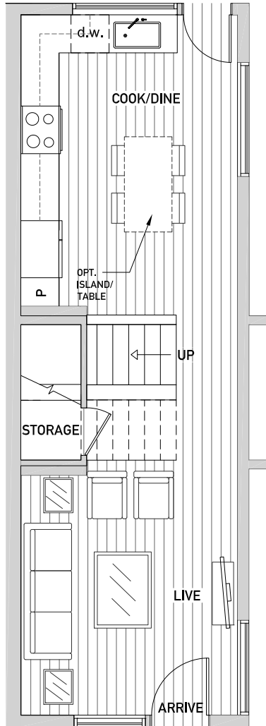
Floor One
