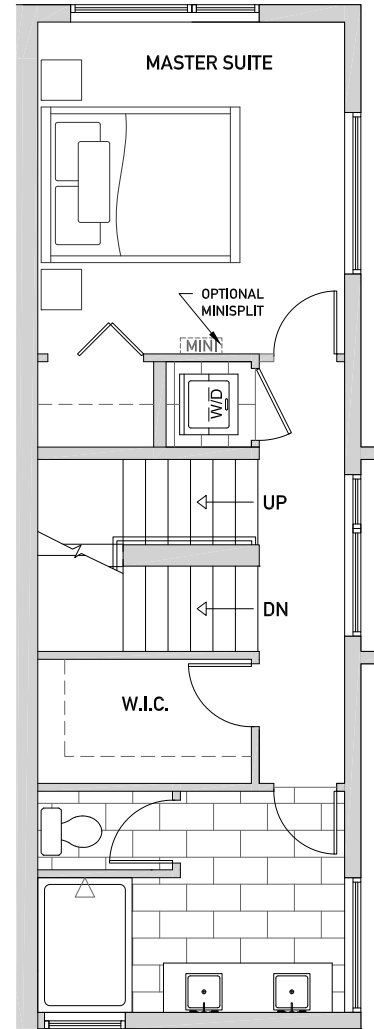
Floor Three
