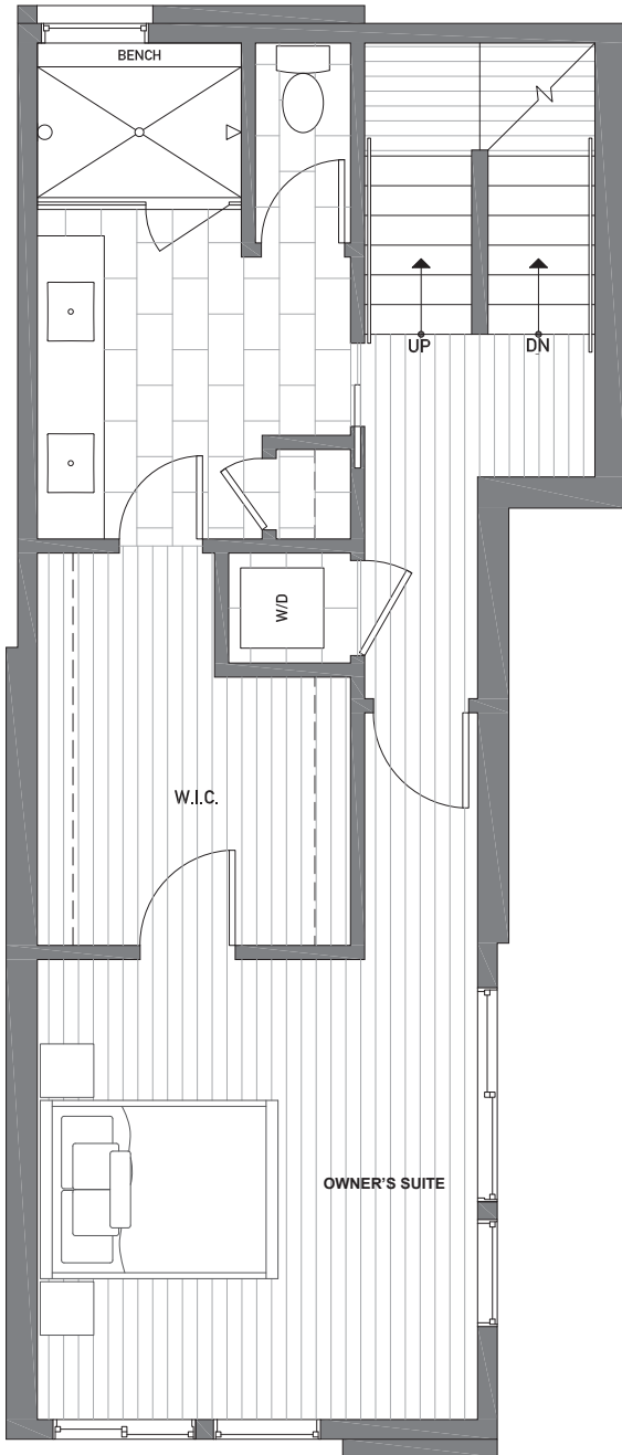
THIRD FLOOR
