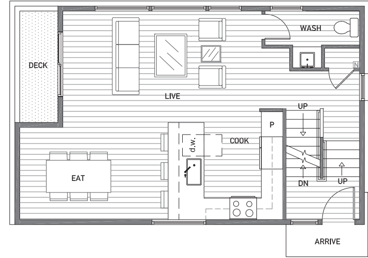
Floor Two
