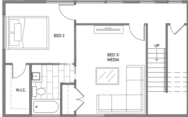
Floor One
