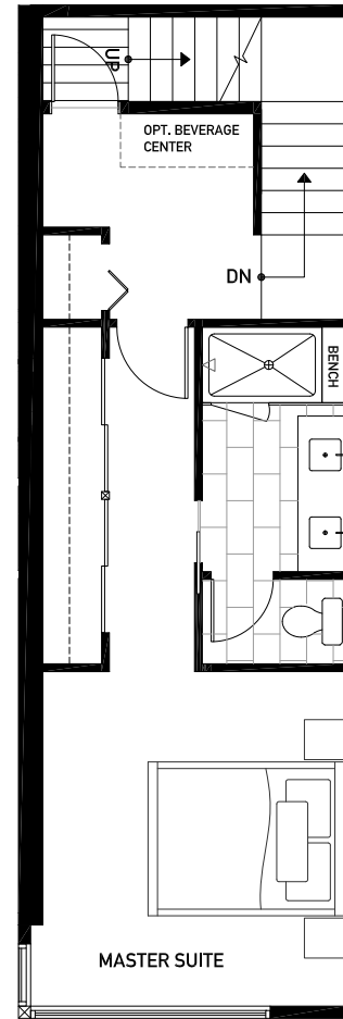
Floor Three
