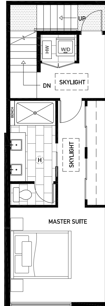
Floor Three
