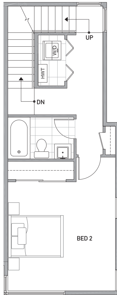
Floor Two
