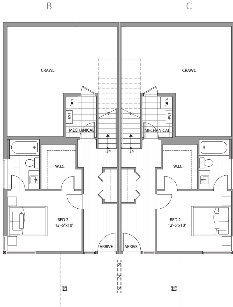
Floor One
