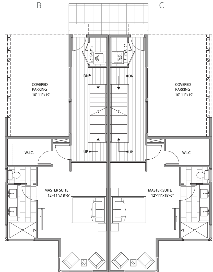
Floor Two
