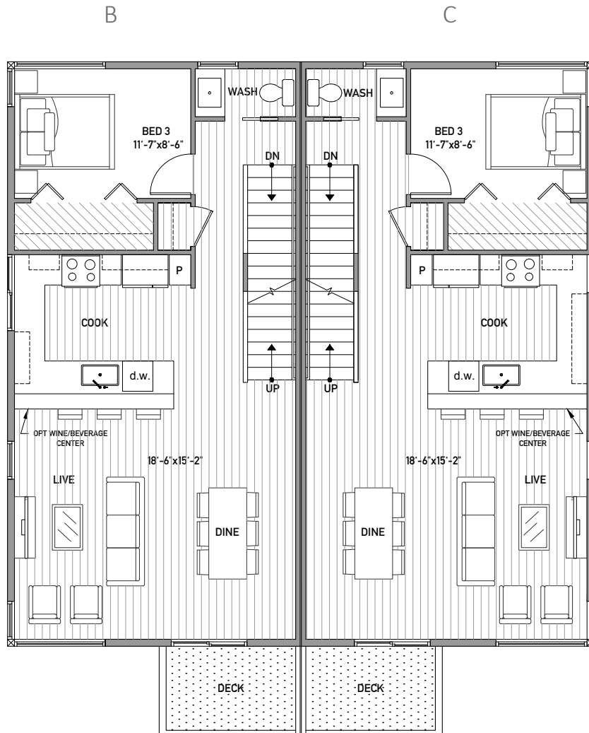
Floor Three
