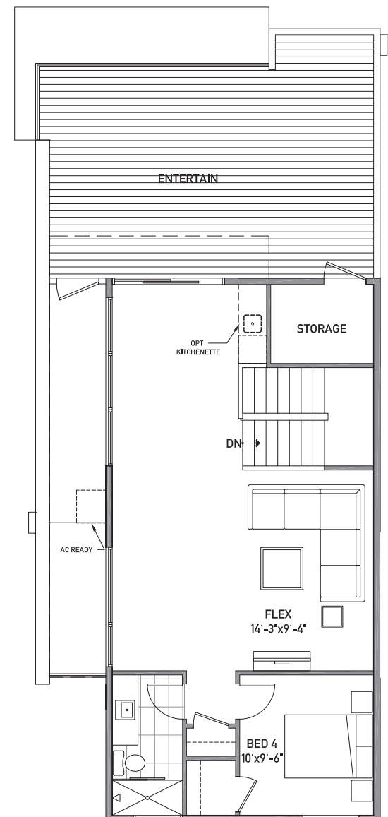
Floor Three
