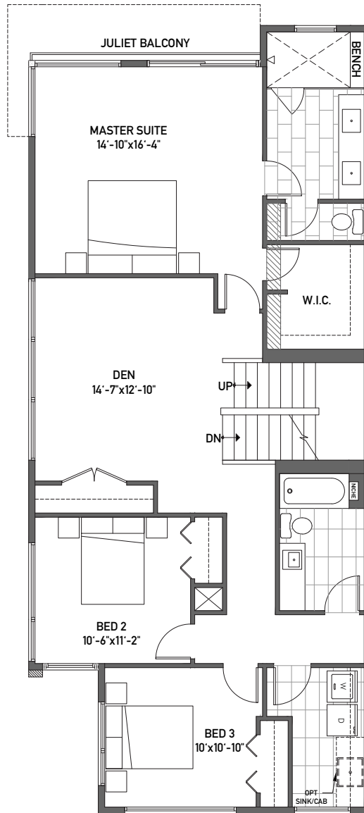
Floor Two
