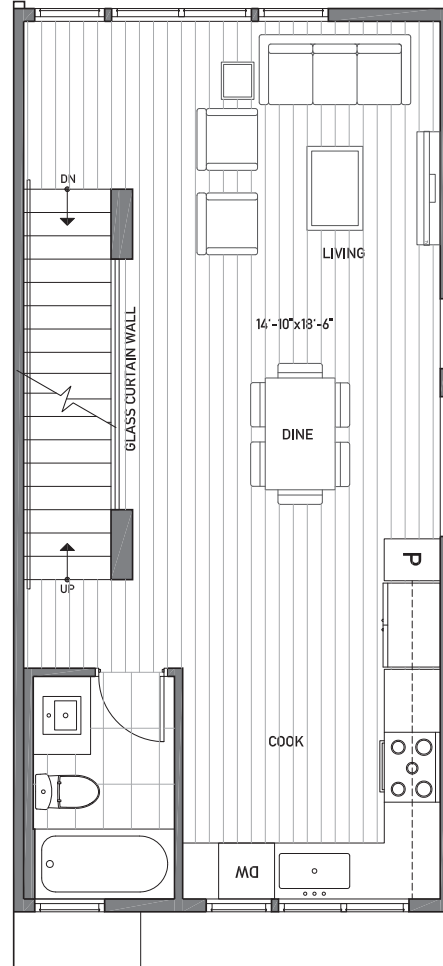
Floor Two
