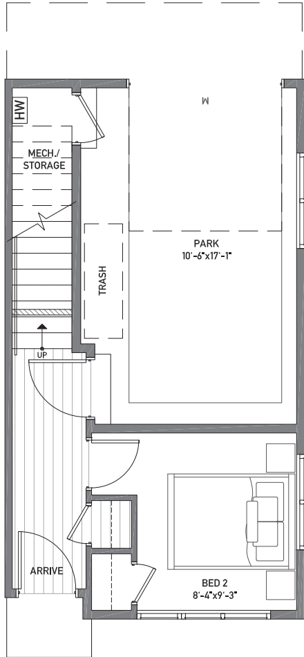
Floor One
