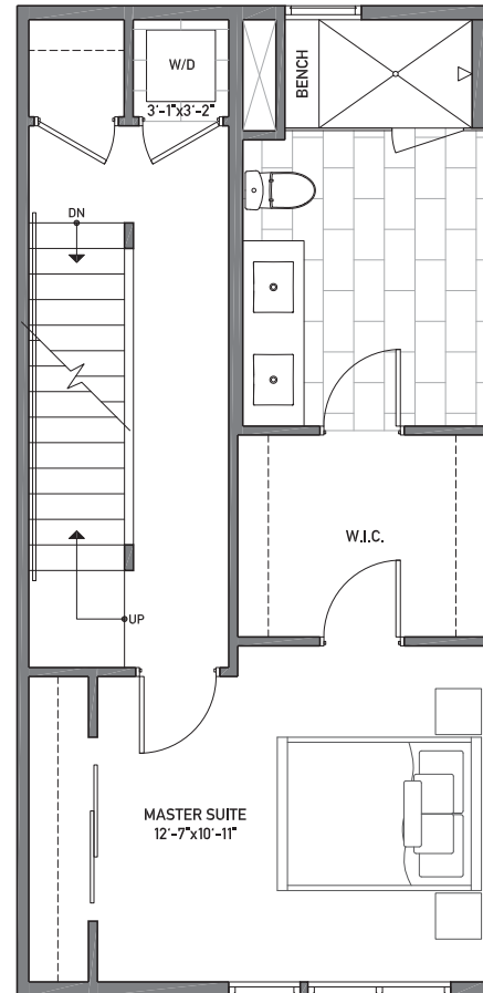
Floor Three
