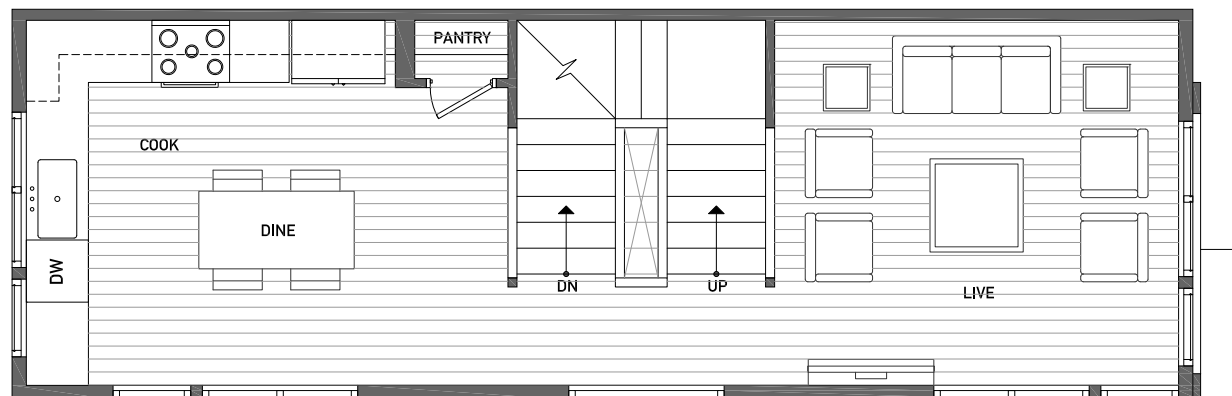
SECOND FLOOR
