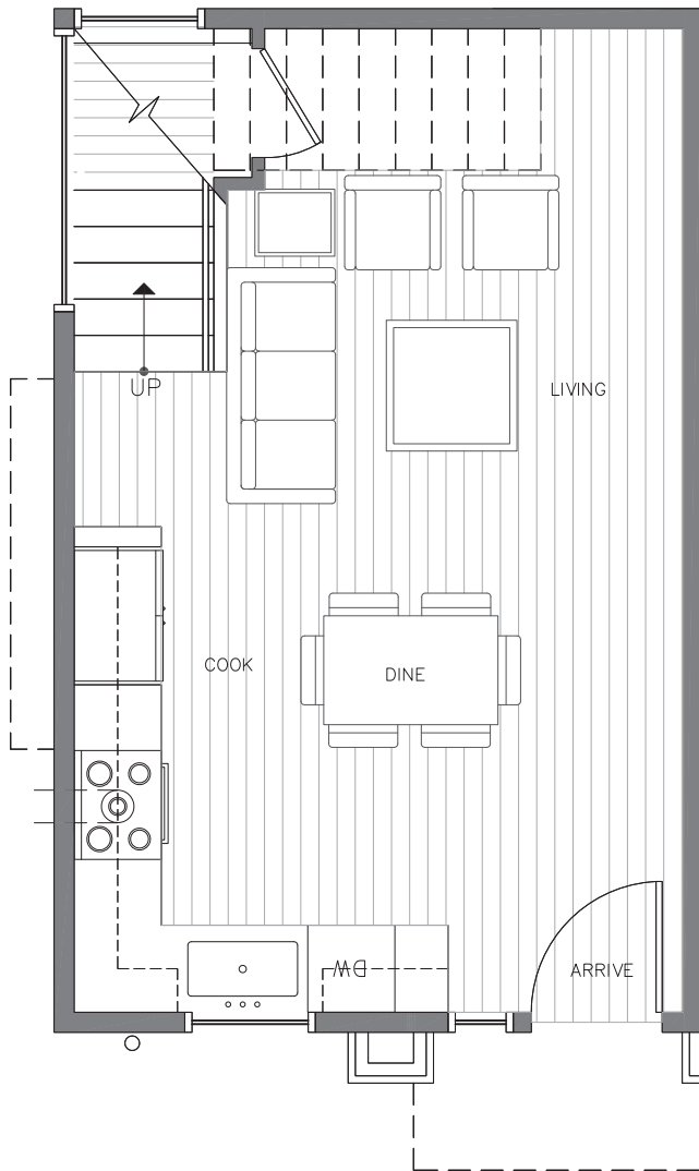
FIRST FLOOR
