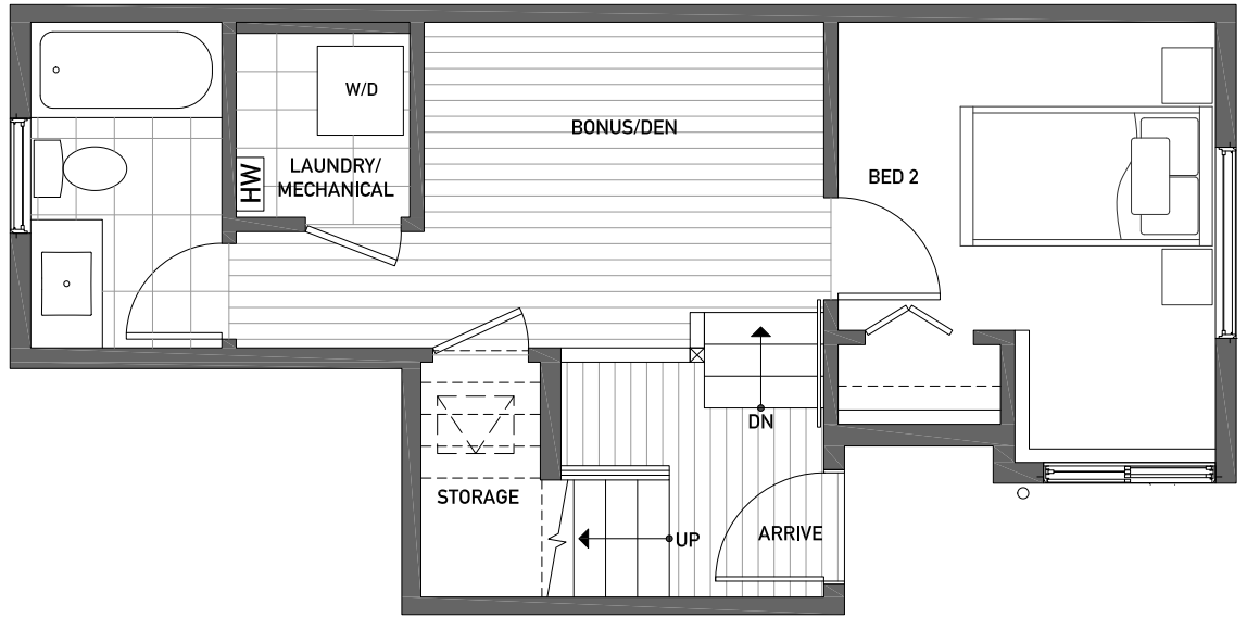
FIRST FLOOR
