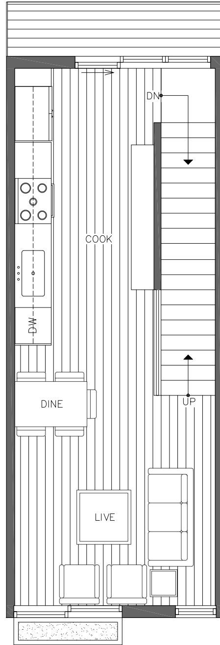
SECOND FLOOR
