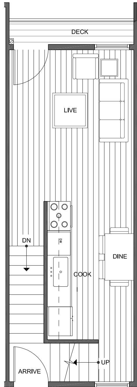
SECOND FLOOR
