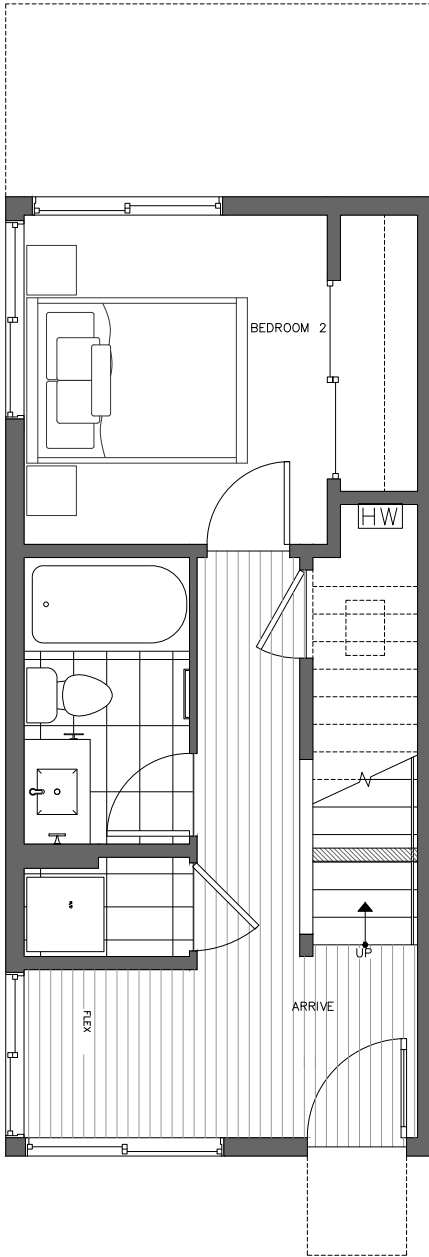
FIRST FLOOR
