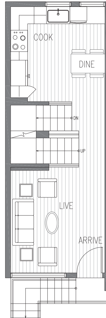
SECOND FLOOR
