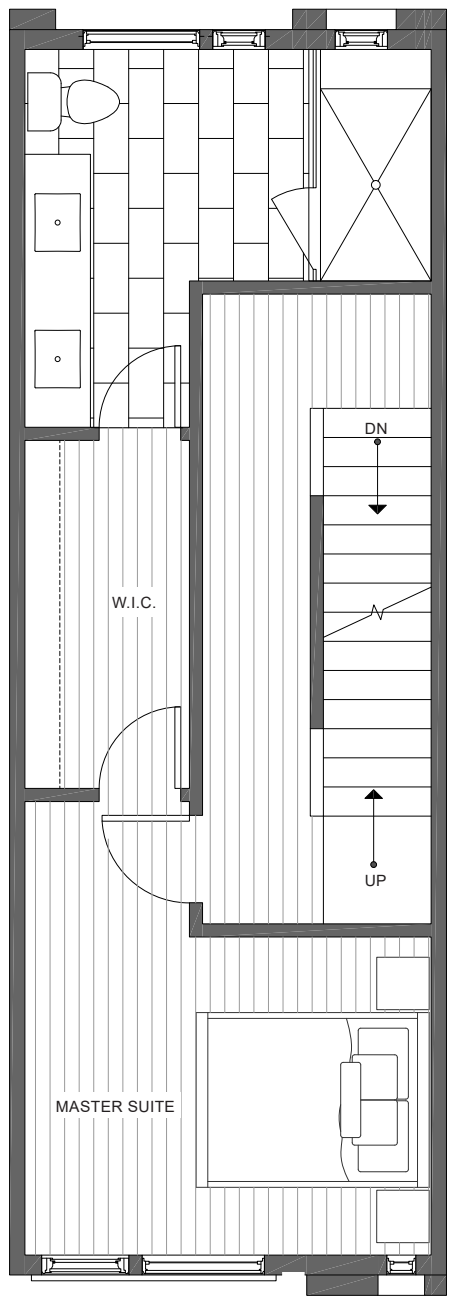
THIRD FLOOR
