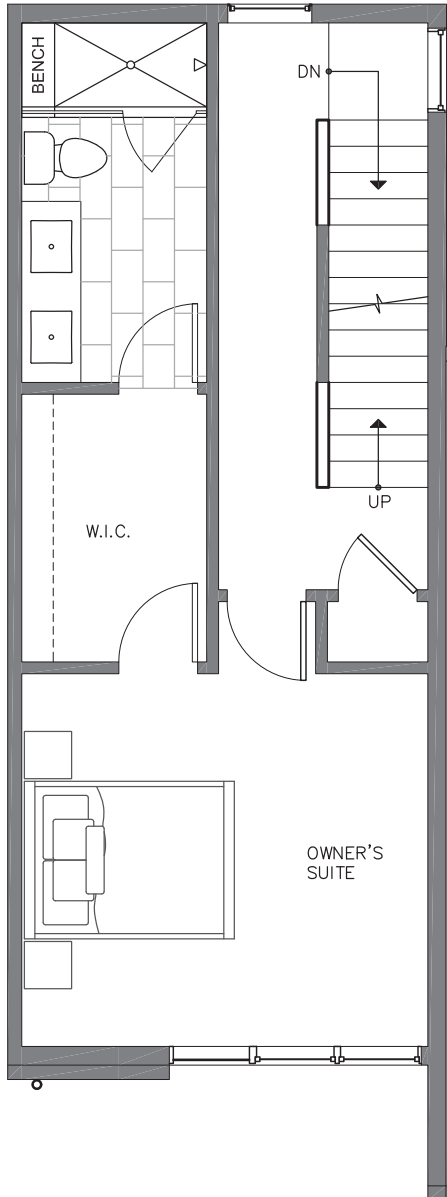
THIRD FLOOR
