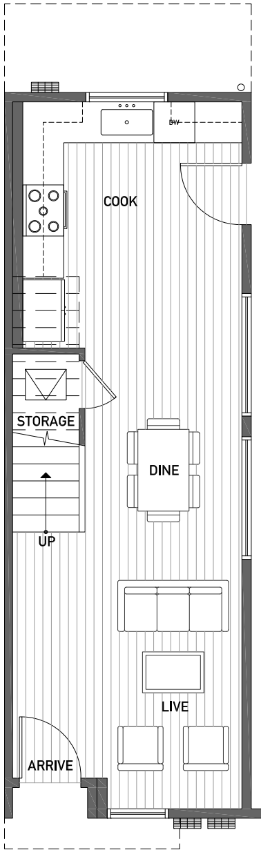
FIRST FLOOR
