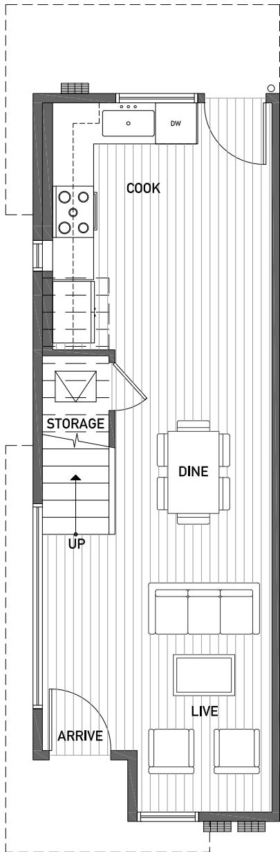
FIRST FLOOR
