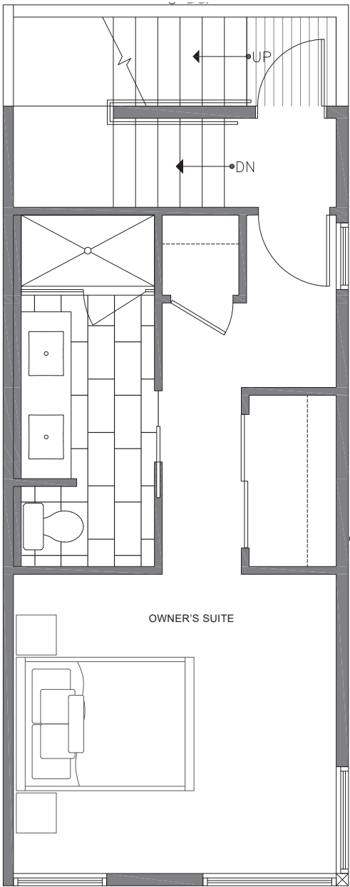
THIRD FLOOR
