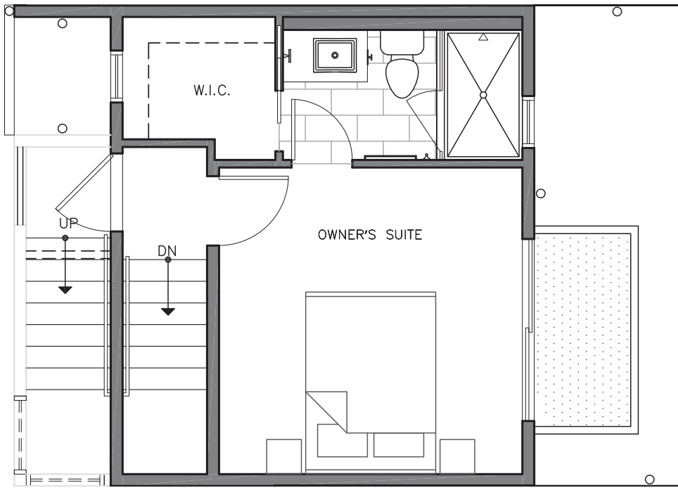
THIRD FLOOR
