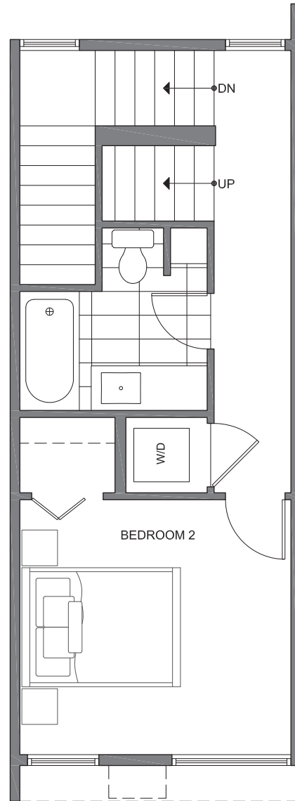
SECOND FLOOR
